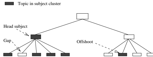
Fig. 3: Three types of features in mapping of a subject cluster to the taxonomy.
