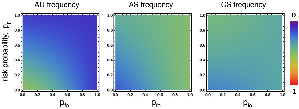
Figure 6. Distant AIS regime. Frequency of AU, AS and CS as a function of the probability of unsafe development being found out, p_{fo} , and the probability of AI disaster occurring p_r , when the number of development steps to reach AIS is very large ( W = 10^6 ). AU has a low frequency whenever p_{fo} or p_r are sufficiently high. AS performs best when p_{fo} is large. Parameters: c = 1 , b = 4 , s = 1.5 , B = 10000 , \beta = 0.01 , population size, Z = 100 .
