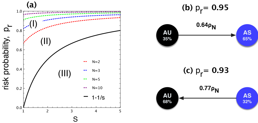
Figure 12. Dotted lines indicate the condition in Equation 24 for different values of group size N . The solid black line indicates the condition in 22. The larger N the larger the region II and smaller the region I. In panels (b), (c): N = 5 . Other parameters: c = 1, b = 4, W = 100, s = 1.5, p_{fo} = 0.5, B = 10000, Z = 100 .
