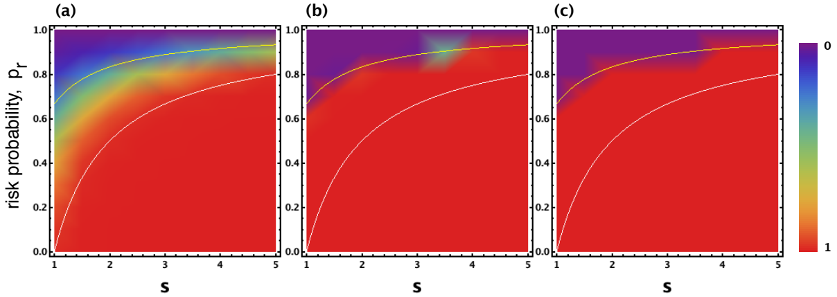
Figure 7. Frequency of AU in a population of three strategies, AS, AU, and CS, as a function of the speed gained when ignoring safety, s , and the risk probability p_r . In general, we observe that when the risk probability is small, AU is dominant. Also, the larger B and s , AU dominates for a larger range. The two solid lines inside the plots indicate the boundaries p_r \in [1 - 1/(3s), 1 - 1/s] where safety development is preferred but non-safety development is preferable (risk-dominant against CS and AS). The observations are valid for varying the selection intensities: \beta = 0.001, 0.01, 0.1 for panels (a), (b) and (c), respectively. Other parameters: c = 1, b = 4, W = 100, p_{fo} = 0.5, B = 10000 , population size, Z = 100 .
