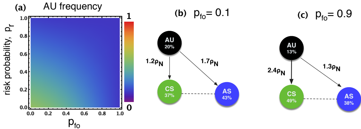
Figure 3. Distant AIS regime. (a) Frequency of AU as a function of the probability of unsafe development being found out, p_{fo} , and the probability of AI disaster occurring p_r , when the number of development steps to reach AIS is very large ( W = 10^6 ). AU has a low frequency whenever p_{fo} or p_r are sufficiently high. (b-c): transition probabilities and stationary distribution ( p_r = 0.75 ). Against AU, AS performs better than CS when p_{fo} is large, which is reversed when p_{fo} is small. Parameters: c = 1 , b = 4 , s = 1.5 , B = 10000 , \beta = 0.01 , population size, Z = 100 .
