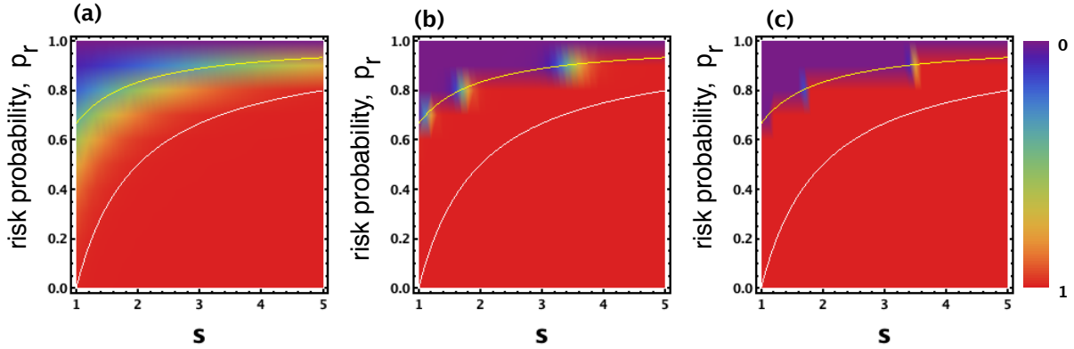
Figure 8. Frequency of AU in a population of two strategies, AS and AU, as a function of the speed gained when ignoring safety, s , and the risk probability p_r . In general, we observe that when the risk probability is small, AU is dominant. Also, the larger B and s , AU dominates for a larger range. The two solid lines inside the plots indicate the boundaries p_r \in [1 - 1/(3s), 1 - 1/s] where safety development is preferred but non-safety development is preferable (risk-dominant against CS and AS). The observations are valid for varying the selection intensities: \beta = 0.001, 0.01, 0.1 for panels (a), (b) and (c), respectively. Other parameters: c = 1, b = 4, W = 100, p_{fo} = 0.5, B = 10000 , population size, Z = 100 .
