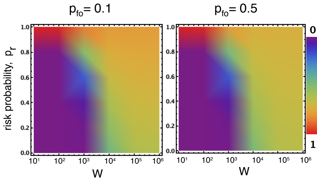
Figure 11. Different regimes of AGI: near AI (small W ) vs distant AGI (large W ). Frequency AU in a population of the three strategies AS, AU and CS in co-presence, as a function of p_r and W . Other parameters: c = 1 , b = 4 , W = 100 , s = 1.5 , p_r = 0.75 , B = 10000 , N = 5 , Z = 100 , \beta = 0.1 .
