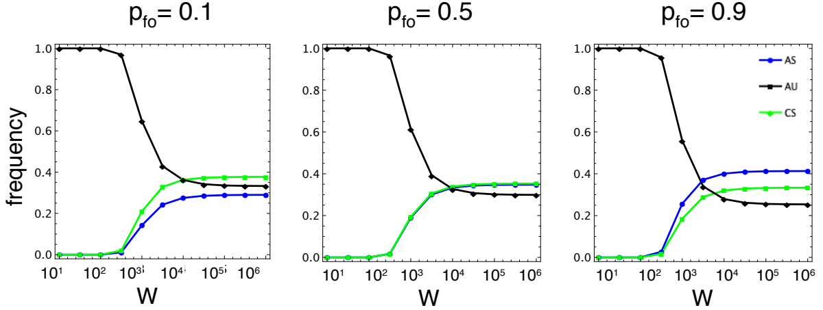
Figure 10. Different regimes of AGI: near AI (small W ) vs distant AGI (large W ). Frequency of AS, AU and CS in a population of the three strategies in co-presence. Other parameters: c = 1 , b = 4 , W = 100 , s = 1.5 , p_r = 0.75 , B = 10000 , N = 5 , Z = 100 , \beta = 0.1 .
