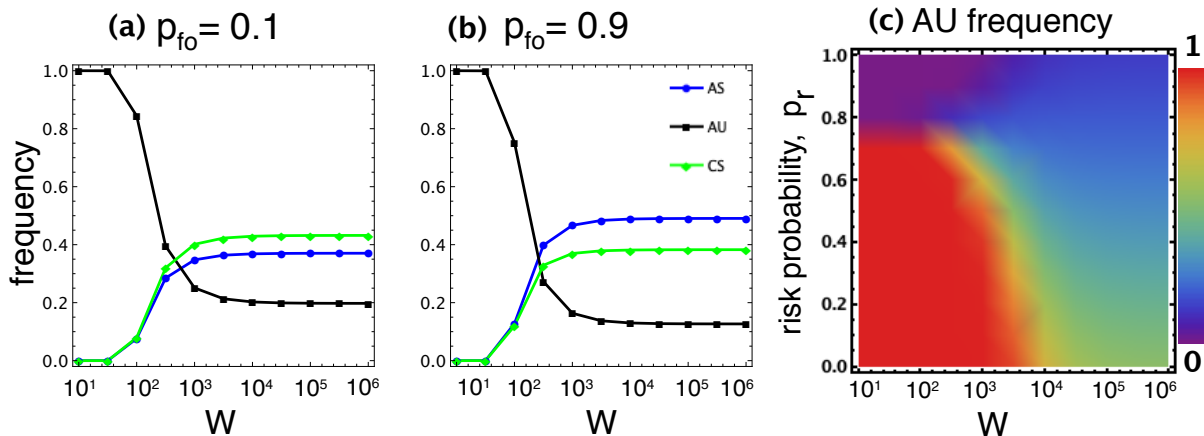
Figure 1. Different regimes of AIS: when W is small (near AIS) vs when W is large (distant AIS). Panels (a) and (b) show the frequency of each strategy in a population of AS, AU and CS ( p_r = 0.75 ). In the near AIS regime, AU dominates the population, while AS and CS outperform AU in the distant AIS regime. This observation is valid for sufficiently small p_r , see panel (c) ( p_{fo} = 0.1 ). For a high risk probability of disaster occurring due to ignoring safety precautions (high p_r ), AU has a low frequency in both regimes. Parameters: c = 1 , b = 4 , W = 100 , B = 10000 , \beta = 0.01 , population size, Z = 100 .
