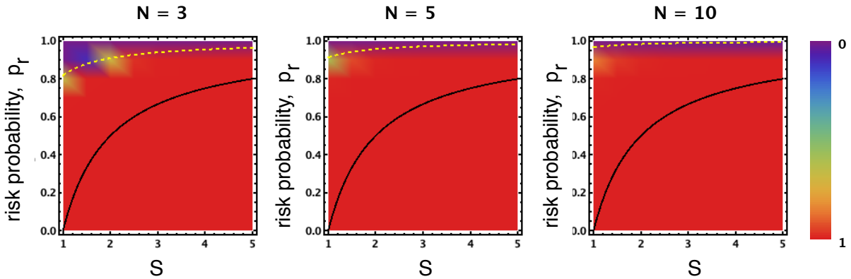
Figure 13. Frequency of AU as a function of the speed gained, s , and the probability of AI disaster occurring p_r , when ignoring safety. Other parameters: c = 1, b = 4, W = 100, s = 1.5, p_{fo} = 0.5, B = 10000, Z = 100 .
